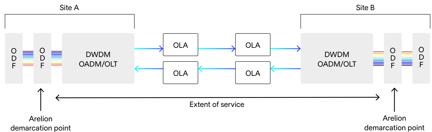
Figure 1: DWDM network components
